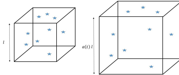
Figure 1: Non-relativistic matter in an expanding universe.
