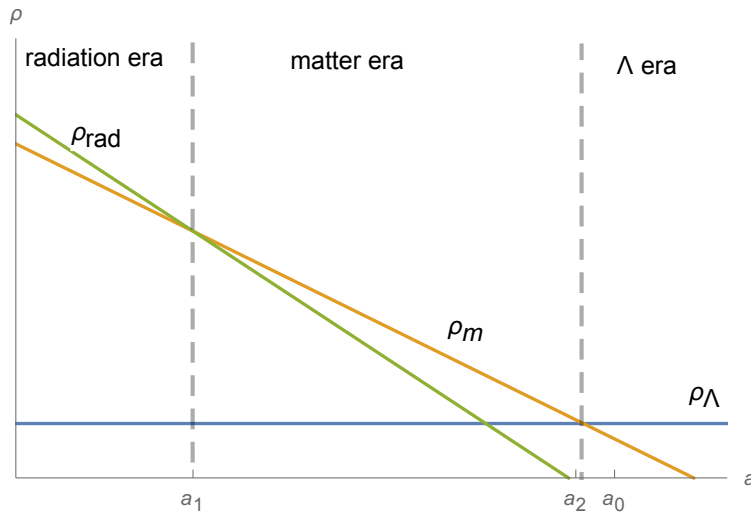
Figure 2: The evolution of our universe.
